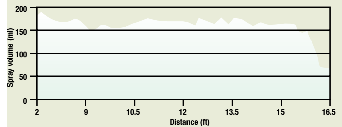
Typical spray pattern produced by the XT Series
